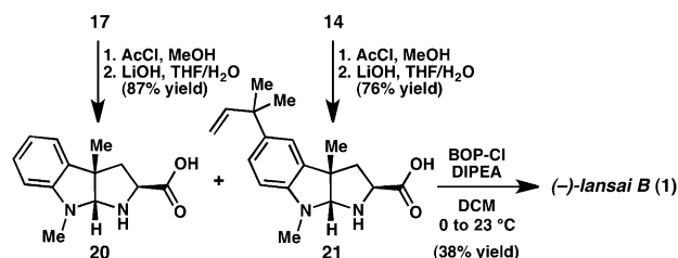
Scheme 2. Synthesis of (–)-lansai B ( 1 ). BOP-Cl = bis(2-oxo-3-oxazolidinyl) phosphonic chloride, DIPEA = N,N -diisopropylethylamine.
