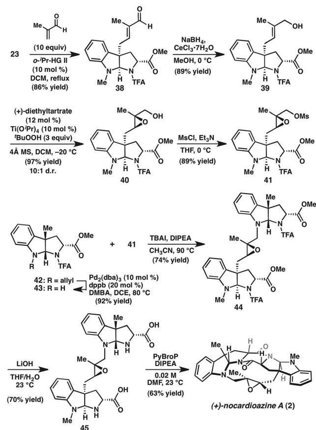
Scheme 5. Synthesis of (+)-nocardiozine A ( 2 ). DMF = N,N -dimethylformamide, MS = molecular sieves, PyBroP = bromotripyrrolidinophosphonium hexafluorophosphate.
