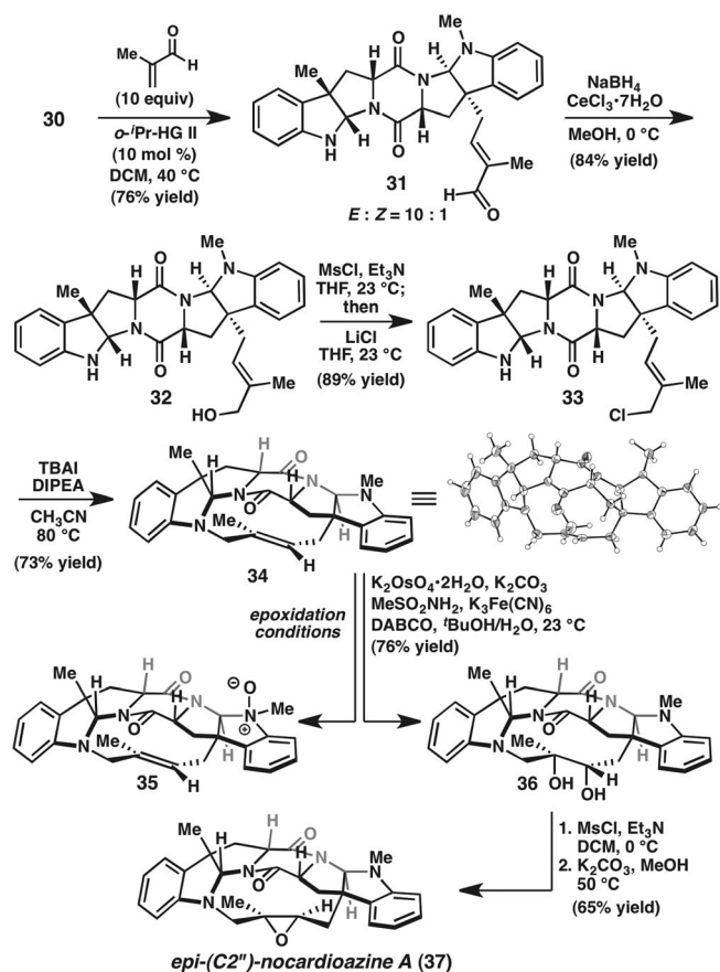
Scheme 4. Synthesis of the nocardiozine A macrocycle. Atomic displacement parameters shown at 50% probability. [13] DABCO = 1,4-diazabicyclo[2.2.2]octane, MsCl = methanesulfonyl chloride, TBAI = tetrabutylammonium iodide.
